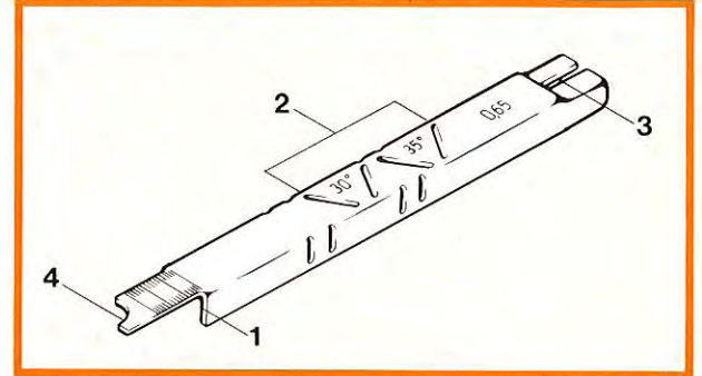
STIHL filing gauge 1 = Sighting edge for side plate angle 2 = Slots for filing angles 3 = Cut-out for depth gauge setting 4 = Groove cleaner and scale for groove depth
